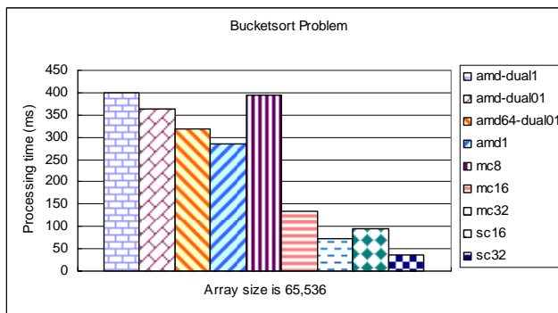
Fig. 23. Comparison of the bucket sort problem when the sizes are equal to 65,536
