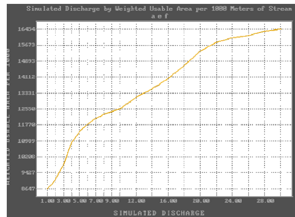
圖8. 流量-WUA關係圖(埔里中華爬岩鯪) Figure 8. Relationship between discharges and WUA . (Sinogastromyzon puliensis)
