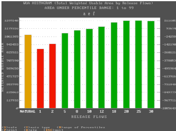
圖5.不同生態放流量之WUA比較圖(埔里中華爬岩鯪) Figure 5. Compared the different ecological release flows of WUA . (Sinogastromyzon puliensis)
